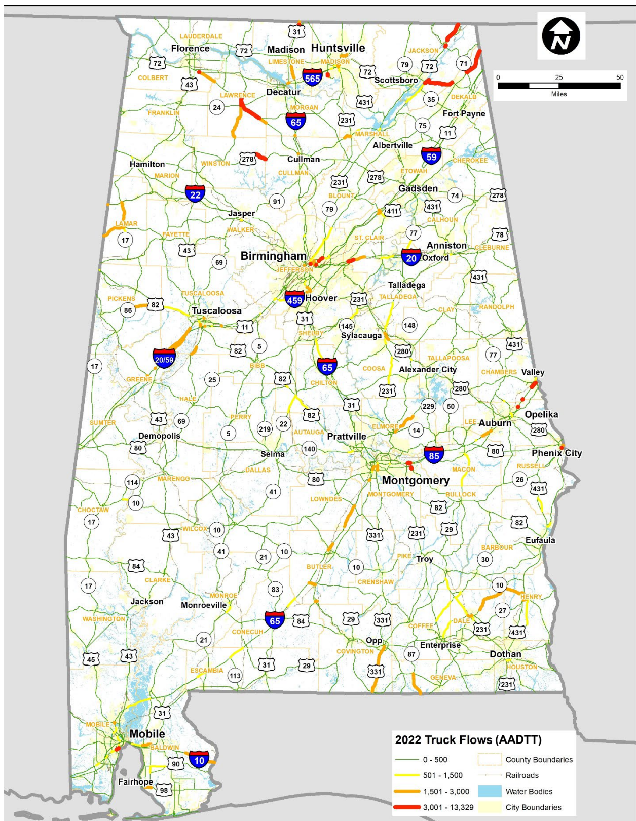
Existing Commodity Flows by Truck (AADTT) (2022)
