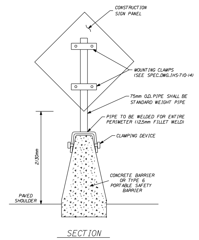
SECTION TEMPORARY SIGN MOUNTING DETAIL
