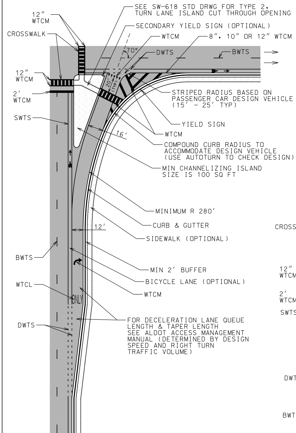
URBAN RIGHT TURN CHANNELIZING LANE WITH DECELERATION LANE (WITH COMPOUND CURB RADII)
