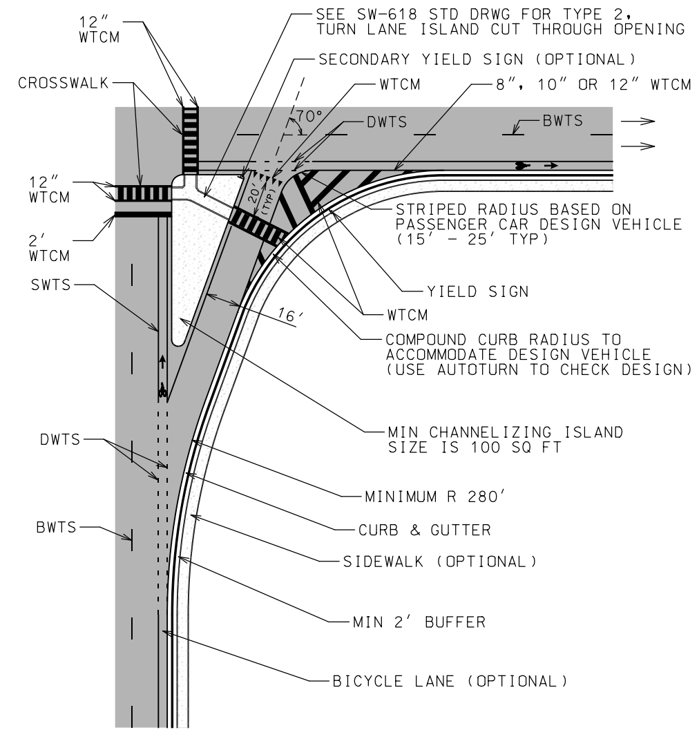
URBAN RIGHT TURN CHANNELIZING LANE WITHOUT DECELERATION LANE (WITH COMPOUND CURB RADII)
