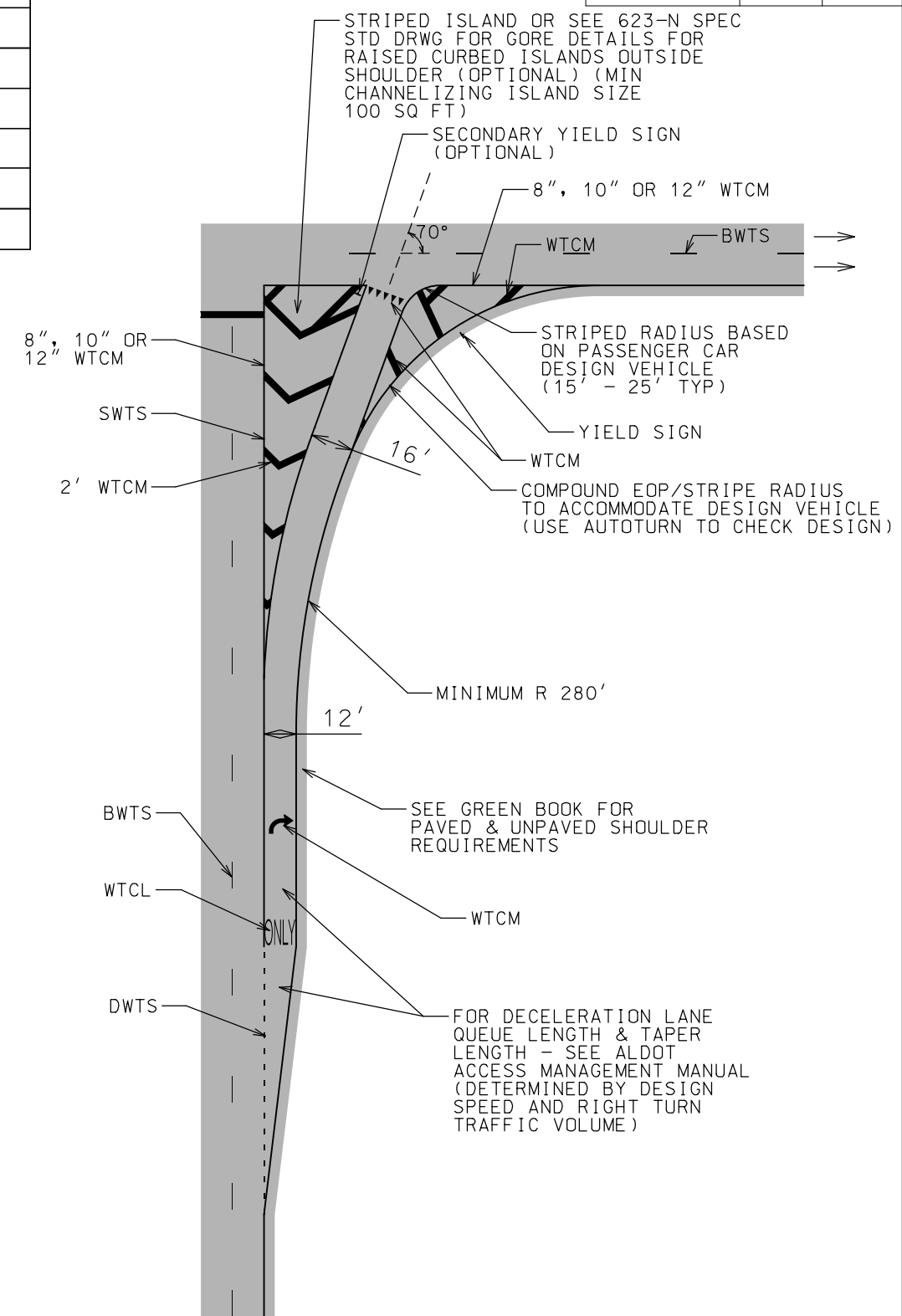
RURAL RIGHT TURN CHANNELIZING LANE WITH DECELERATION LANE (WITH COMPOUND CURB RADII)
