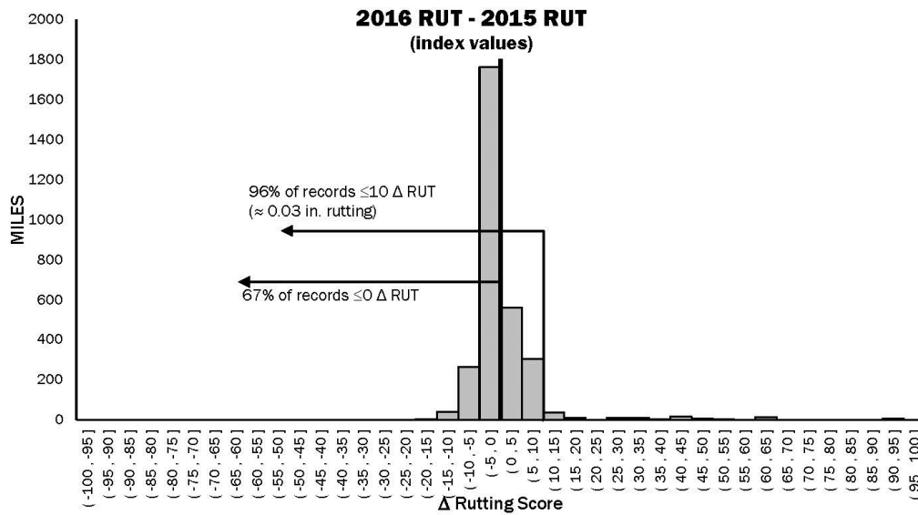
Figure 3. Mileage-based comparison of NHS rutting scores
