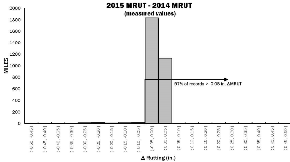
Figure 4. Mileage-based comparison of NHS rutting values
