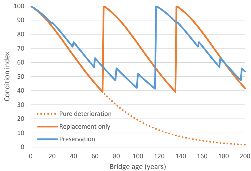
Exhibit 46: Preservation Extends the Service Life of a Typical Alabama Bridge
