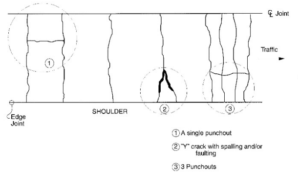
FIGURE 2. PUNCHOUT DEFINITIONS Source: 2003 Distress Identification Manual for the Long-Term Pavement Performance Program
