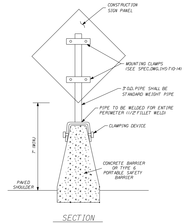
TEMPORARY SIGN MOUNTING DETAIL
