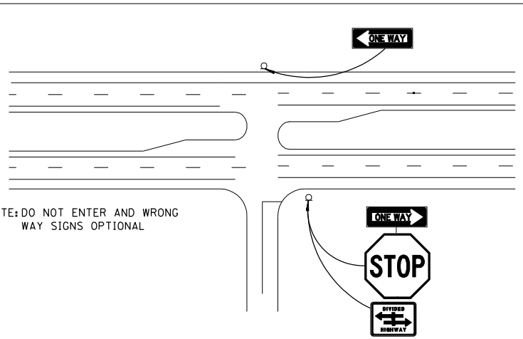
T-INTERSECTION MEDIAN FROM 9 METERS TO 24 METERS
