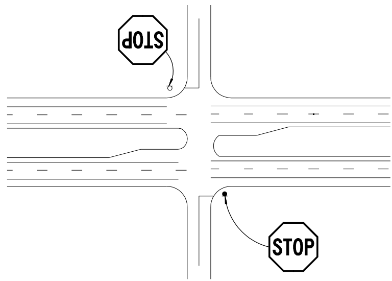
MEDIAN UNDER 9 METERS FOR A CROSSROAD
