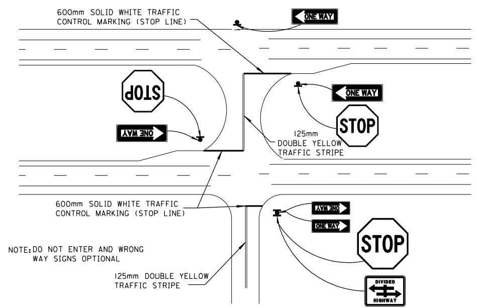
T-INTERSECTION MEDIAN OVER 24 METERS
