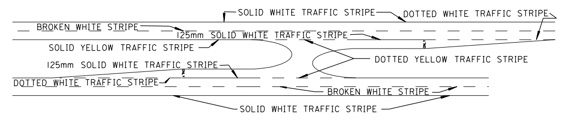
TYPICAL STRIPING DETAIL FOR CROSSOVERS
