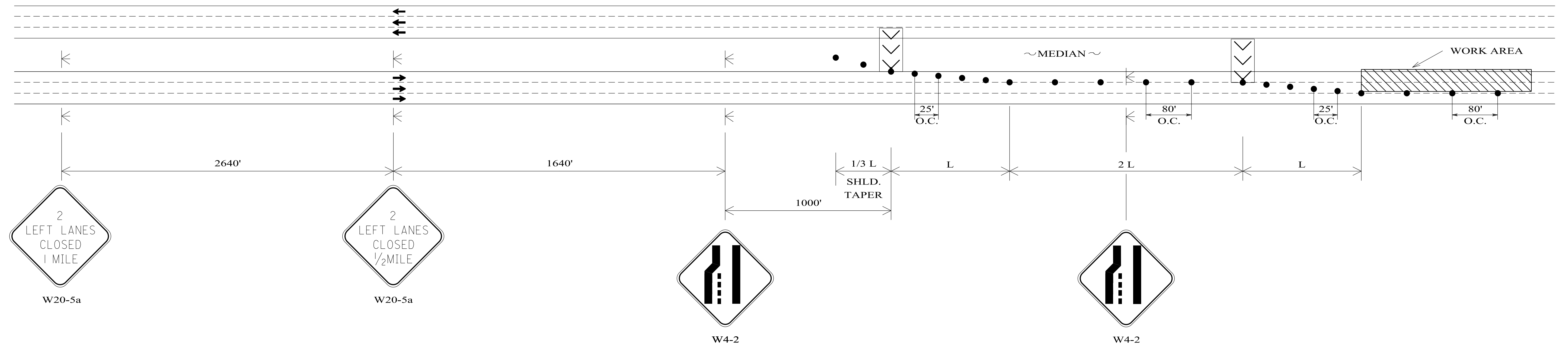
TYPICAL SCHEME FOR DOUBLE LANE CLOSURES (LEFT)
