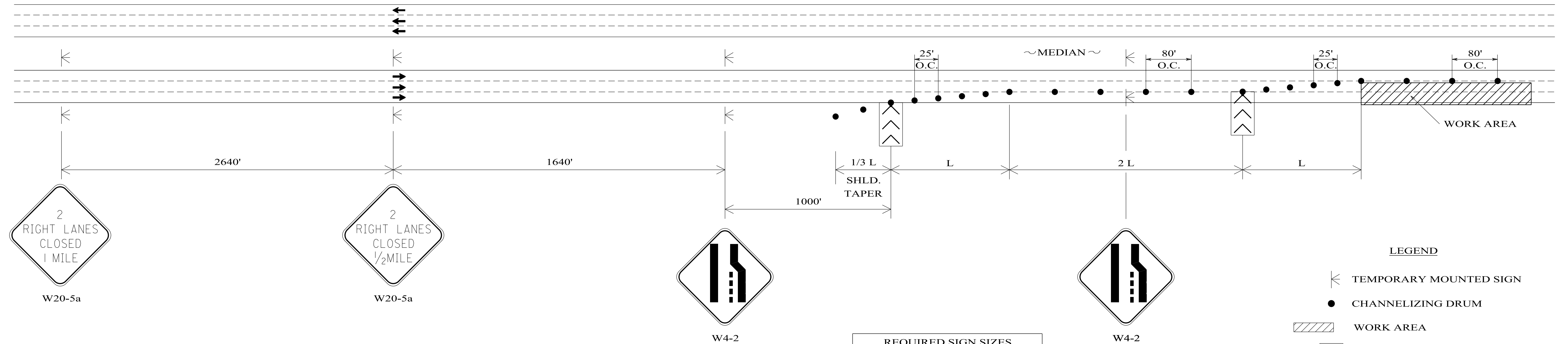
TYPICAL SCHEME FOR DOUBLE LANE CLOSURES (RIGHT)
