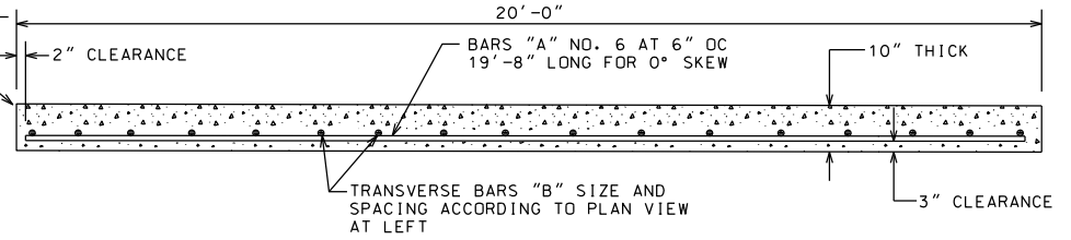
TYPICAL LONGITUDINAL SECTION NOT TO SCALE
