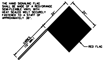
HAND SIGNALING FLAG
