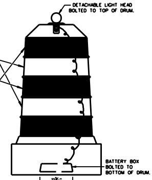
EXAMPLE OF DETACHABLE HEAD WARNING LIGHT ATTACHED TO DRUM
