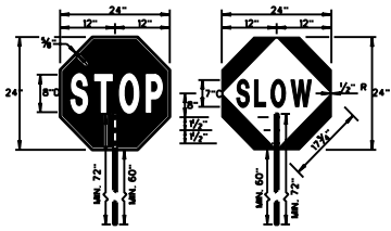
STAFF MOUNTED PADDLES
