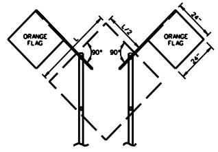
WARNING FLAGS MOUNTING ON CONSTRUCTION SIGNS
