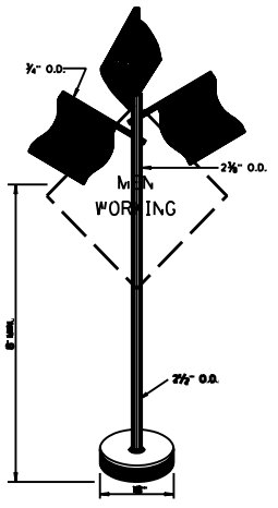
WARNING FLAG UNIT
