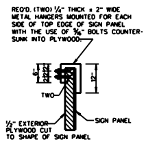
INSTALLATION OF SIGN COVERING MATERIAL DURING NON-USE
