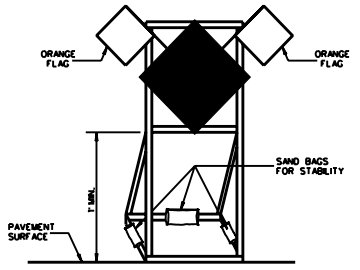
TYPICAL SIGN INSTALLATION (TEMPORARY SUPPORTS)
