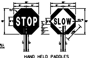
HAND HELD PADDLES
